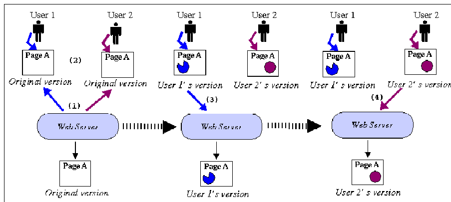
Figure 6. An example of “lost update problem” situation
