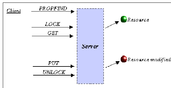
Figure 7. A client/server interaction using HTTP/WebDAV requests
