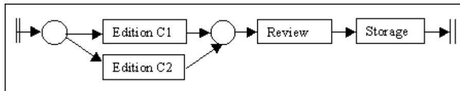
Figure 3. Simple authoring workflow
