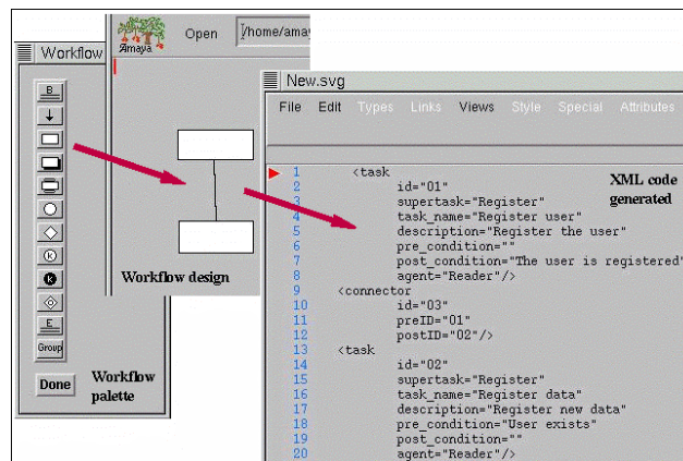
Figure 5. Workflow editor and the XML code produced
